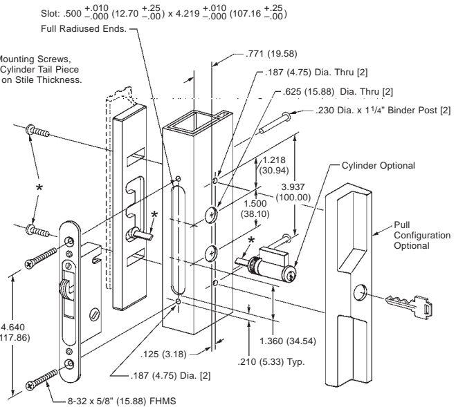
CARTWHEEL FABRICATION—SURFACE MOUNTING ON PVC
