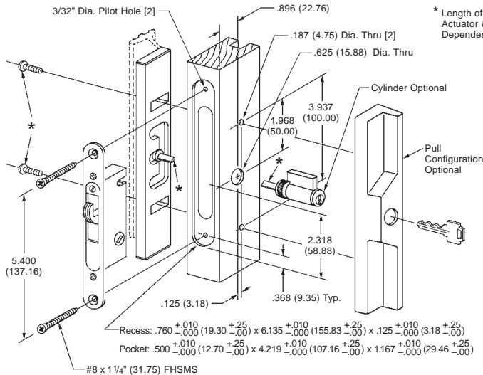
PAGEBOOK FABRICATION—FLUSH MOUNTING ON WOOD
